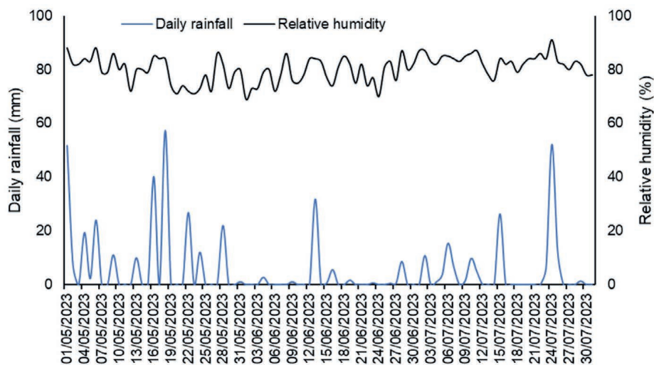
Fig. 1. The daily rainfall and relative humidity at the research site during the research had been conducted. (Source: Indonesian Agency for Meteorology, Climatology and Geophysics).
