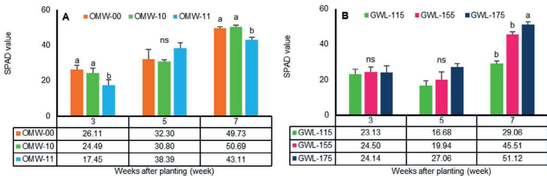
Fig. 5. Comparison of SPAD values under or without organic mulch (A) and at different depths of the groundwater table (B). Each bar followed by the different letter means significantly different at LSD 0.05 . Meanwhile, ns means do not significantly different at LSD 0.05 . OMW-00 = without mulch and watering, OMW-10 = with mulch but no watering, and MWO-11 = with mulch and watering. GWL-115 = with water table at 11.5 cm, GWL-155 = water table at 15.5 cm, and GWL-175 = water table at 17.5 cm below media surface.
